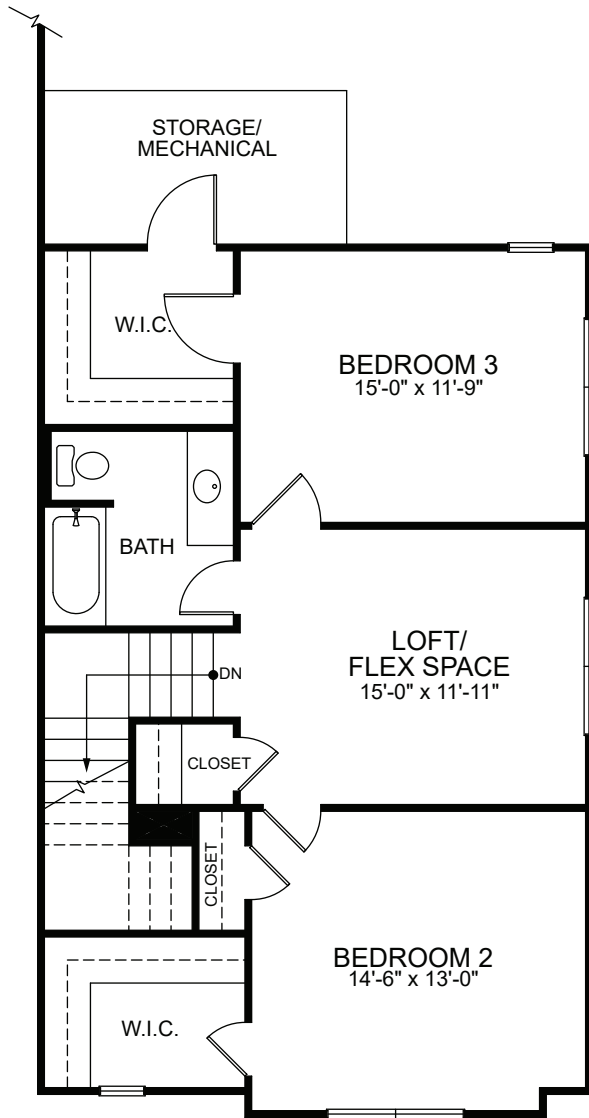
SECOND FLOOR
